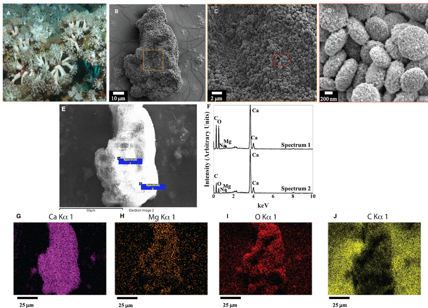
Fig. 1. Ovabunda macrospiculata colony with extended polyps and tentacles (A). SEM images of aggregated O. macrospiculata sclerites (B). Magnified image of microscleres at the surface of the sclerites (C is the inset orange box in B, D is the inset red box on C). EDS mapping of (B) showing the distribution of calcium, magnesium, oxygen, and carbon in the sclerite (G–J). Photo credit for (A): Ronen Liberman, Tel Aviv University. (For interpretation of the references to color in this figure legend, the reader is referred to the web version of this article.)
