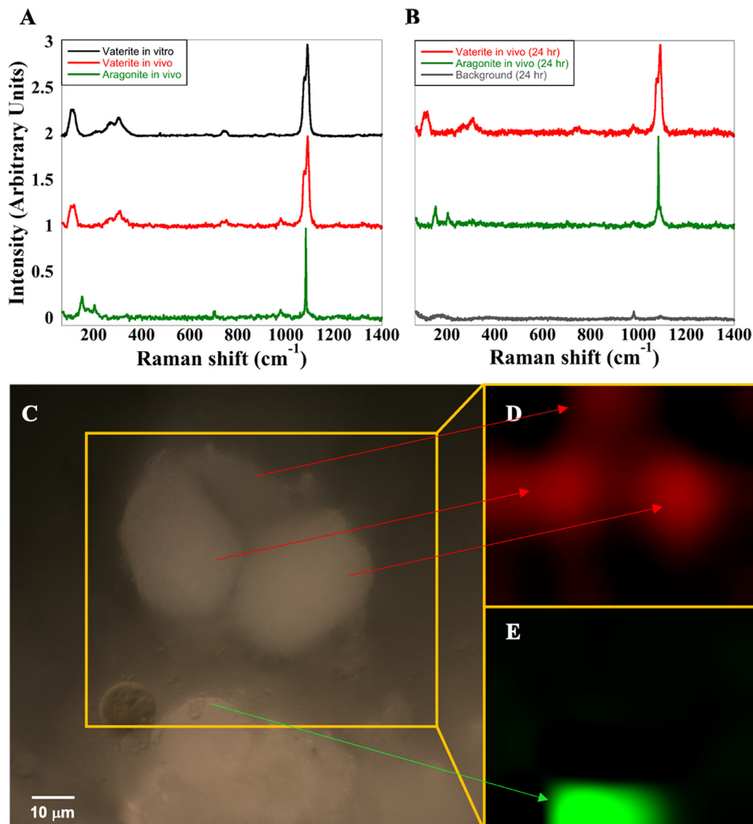
Fig. 2. Micro-Raman spectroscopic mineral determination of isolated (A) and embedded (B) sclerites. (A) Vaterite (black) was observed in a fixed sample of an O. macrospiculata sclerite isolated from the tissue. Vaterite (red) and aragonite (green) were observed in an in-vivo sclerite embedded in live tissue of O. macrospiculata . (B) The same colony was re-examined in-vivo after 24 h, with vaterite (red) and aragonite (green) still detected. A small peak observed at \sim 980\text{ cm}^{-1} in all in-vivo measurements is likely sulfate from the surrounding seawater (panel B, gray spectrum). (C) Light micrograph with mapped locations of vaterite (red, D) and aragonite (green, E) within polyp tissue. D and E are the same locations in C noted by the orange box. Arrows denote specific features of C observed by Raman spectroscopy to be vaterite (D) or aragonite (E) (For interpretation of the references to color in this figure legend, the reader is referred to the web version of this article.).
